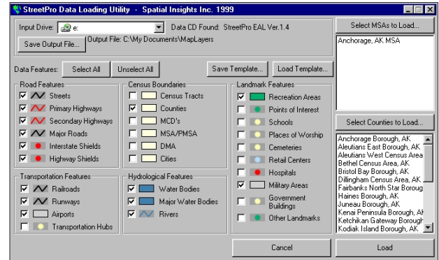
StreetPro™ Extract/Append Program Interface
